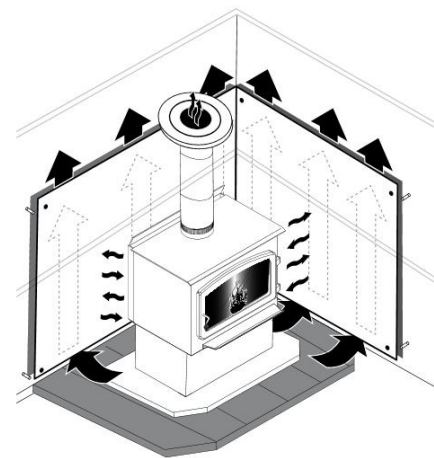
Heat shield
