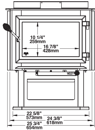
Figure 2: Front view
