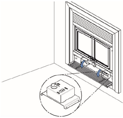
Figure 1: Blower location
