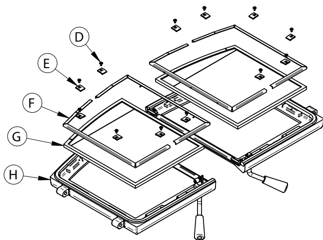
Figure 2: Double door
